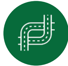
Autocomplete
